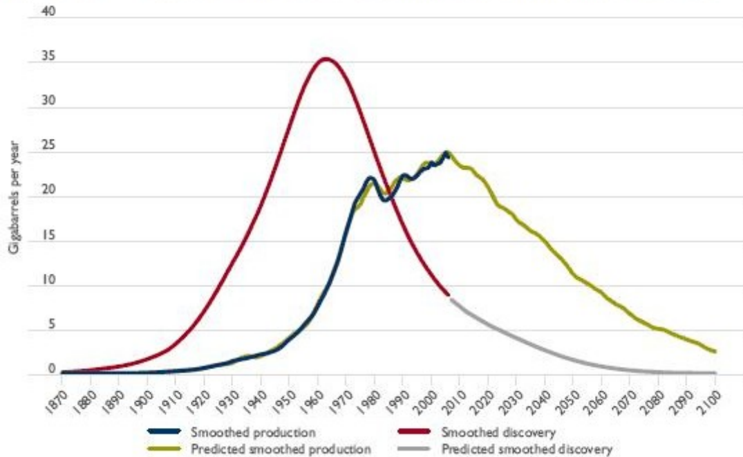
Figure 13.9 Annual world discovery and production of conventional oil
